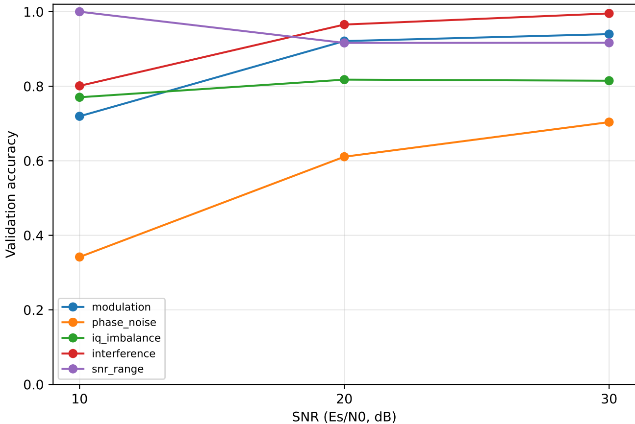
CNN accuracy vs SNR (per task)
